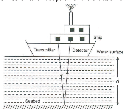
Ultrasound sent by a transmitter and received by a detector.
